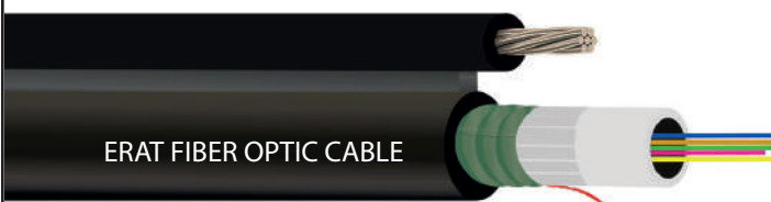
Figure 8 Type, SLT-SJCSA-PE Fiber Optic Cable
