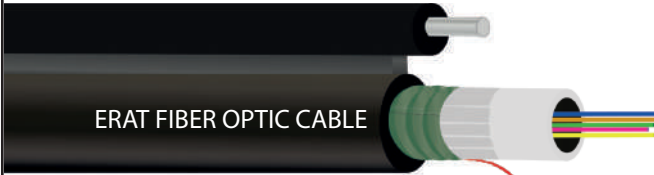
Figure 8 Type, SLT-SJNMA-PE Fiber Optic Cable
